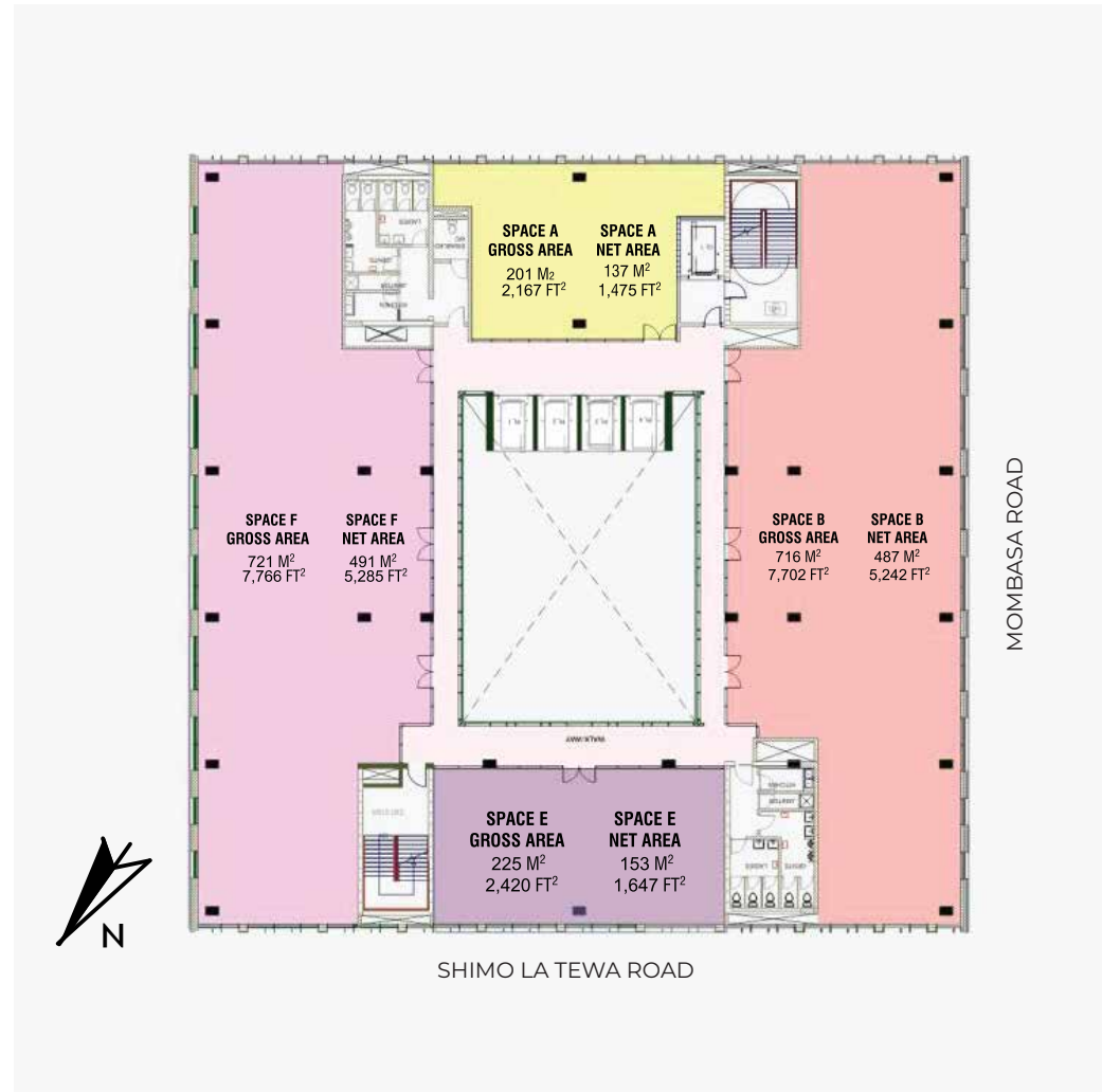
B. TYPICAL FLOOR - 4 SUBDIVISIONS
